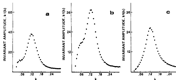
Figure 4. SAXS scans of (a) as-received 1100 EW Nafion, (b) solution-processed 1100 EW Nafion, and (c) recast 1100 EW Nafion. All samples are hydrated Na + form.
