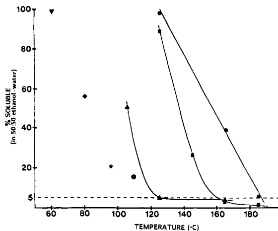
Figure 2. Effect of solvent and evaporation temperature on the solubility of solution-cast Na + form 1100 EW Nafion. Solvents: ▽, 50:50 ethanol-water; ♦, ethanol; ★, propanol; ●, butanol; ▲, DMF; ■, DMSO; ●, EG.
