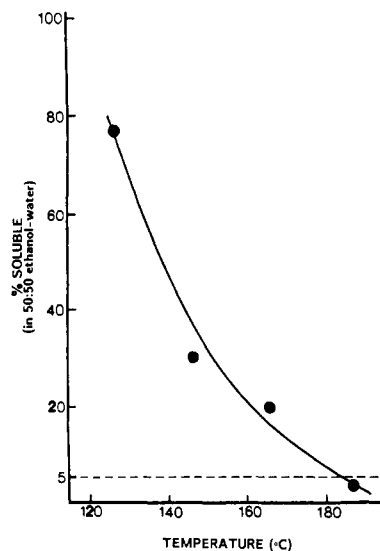
Figure 1. Effect of evaporation temperature on the solubility of solution-cast Na + form Dow PFSI (solvent = DMSO).
