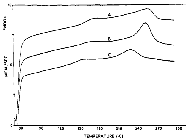
Figure 5. DSC thermograms of (A) as-received 1100 EW Nafion, (B) solution-processed 1100 EW Nafion, and (C) recast 1100 EW Nafion. All samples are Na + form.
