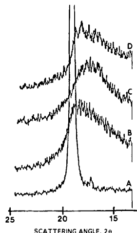
Figure 3. WAXD scans of (A) Teflon, (B) as-received 1100 EW Nafion, (C) recast 1100 EW Nafion, and (D) solution-processed 1100 EW Nafion. All Nafion samples are Na + form.
