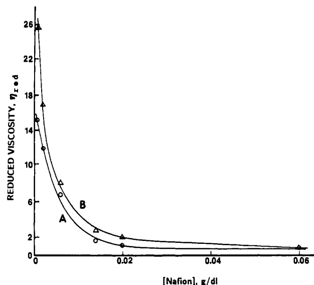
Figure 6. Plots of reduced viscosity vs concentration for 1100 EW Nafion in 50:50 ethanol-water at 25 °C. Curve A is for the unsonicated solutions, and curve B is for the ultrasonicated solutions.
